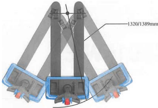
MINI type Electric Pallet Truck turning radius
